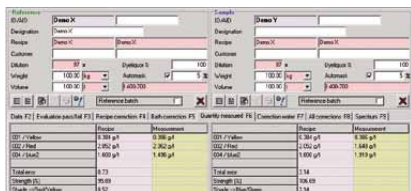
Analysis of the composition of dye liquor
